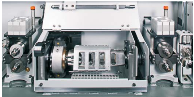
▼ Servo-Adjustable Straightening Rotor (Option)
