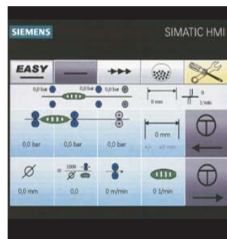
▲ Color touchscreen
