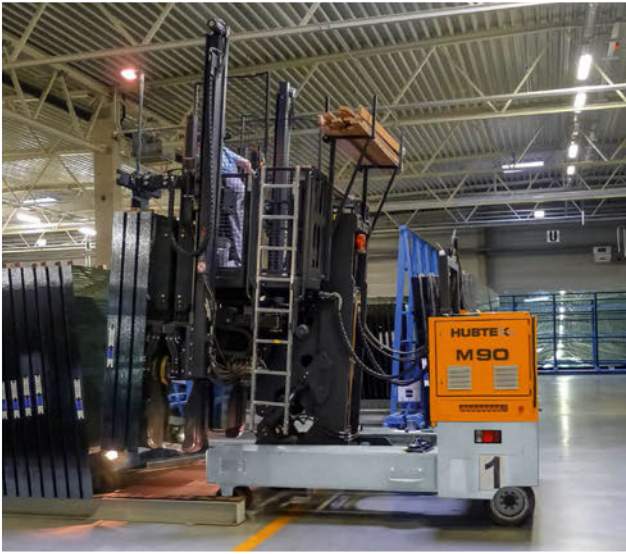
M 90 storing glass packs on floor bearers
